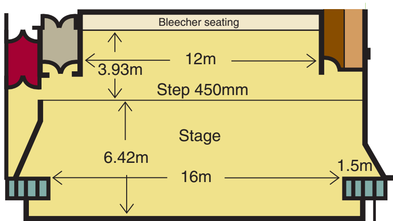
Stage Dimensions
